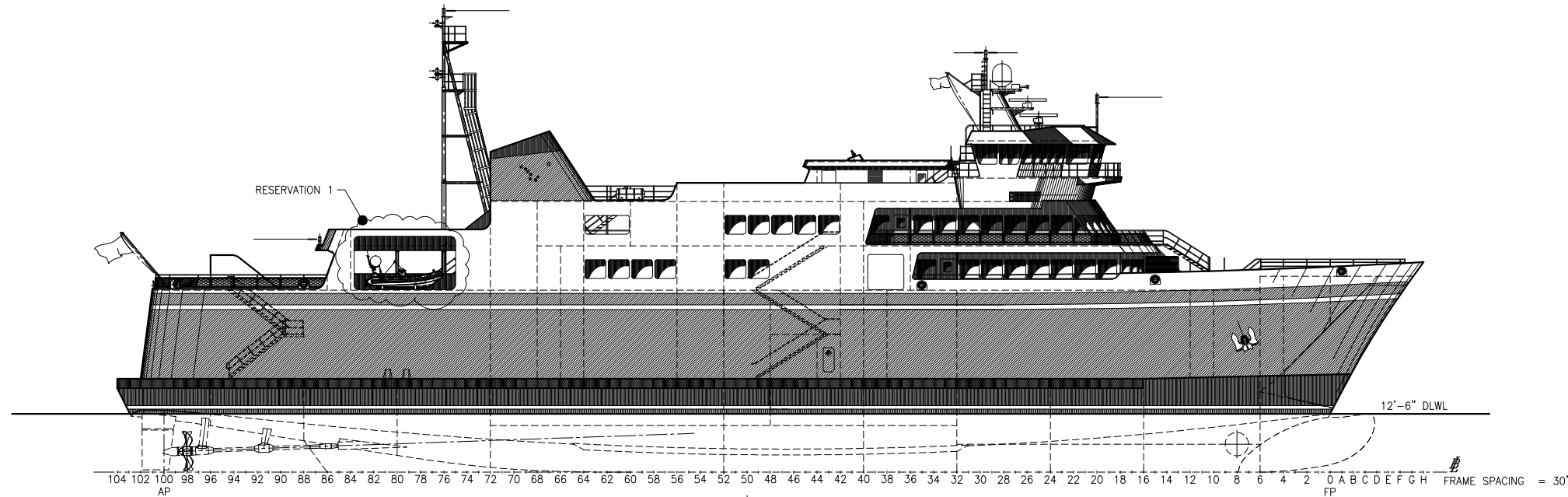
OUTBOARD PROFILE \triangle 1,2,4,5,7,8,9,10,11,11,12
